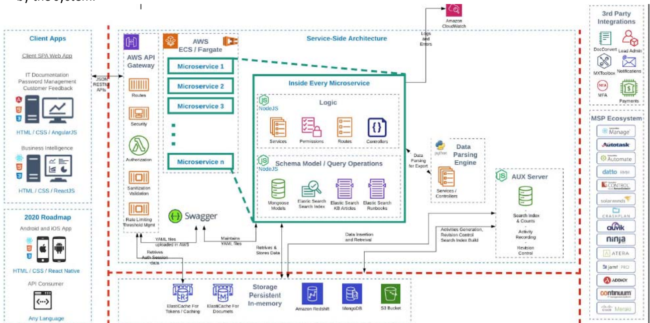
ITBoost System Architecture
